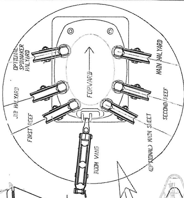
MAST STEP DETAIL
